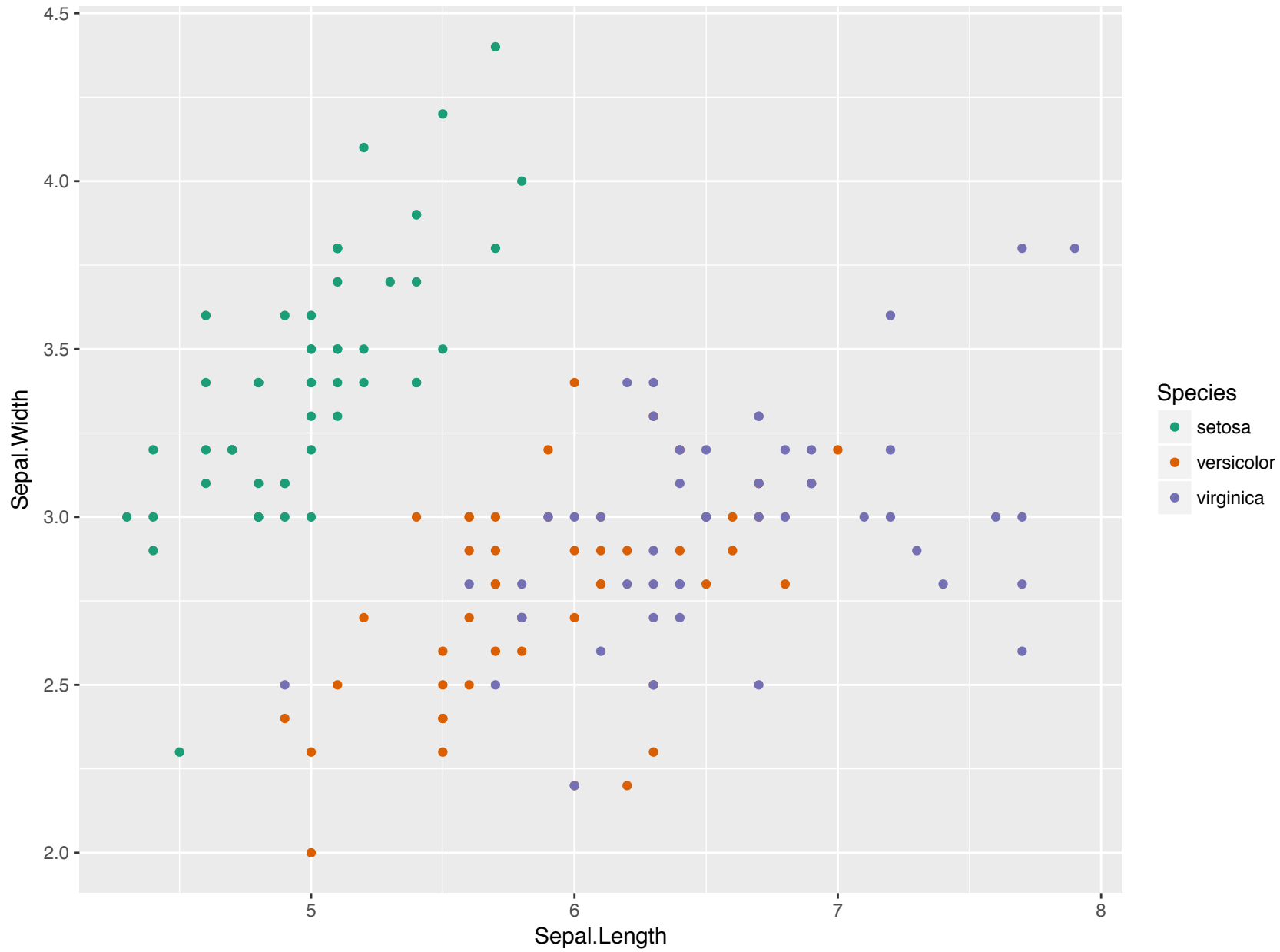
Training Data
