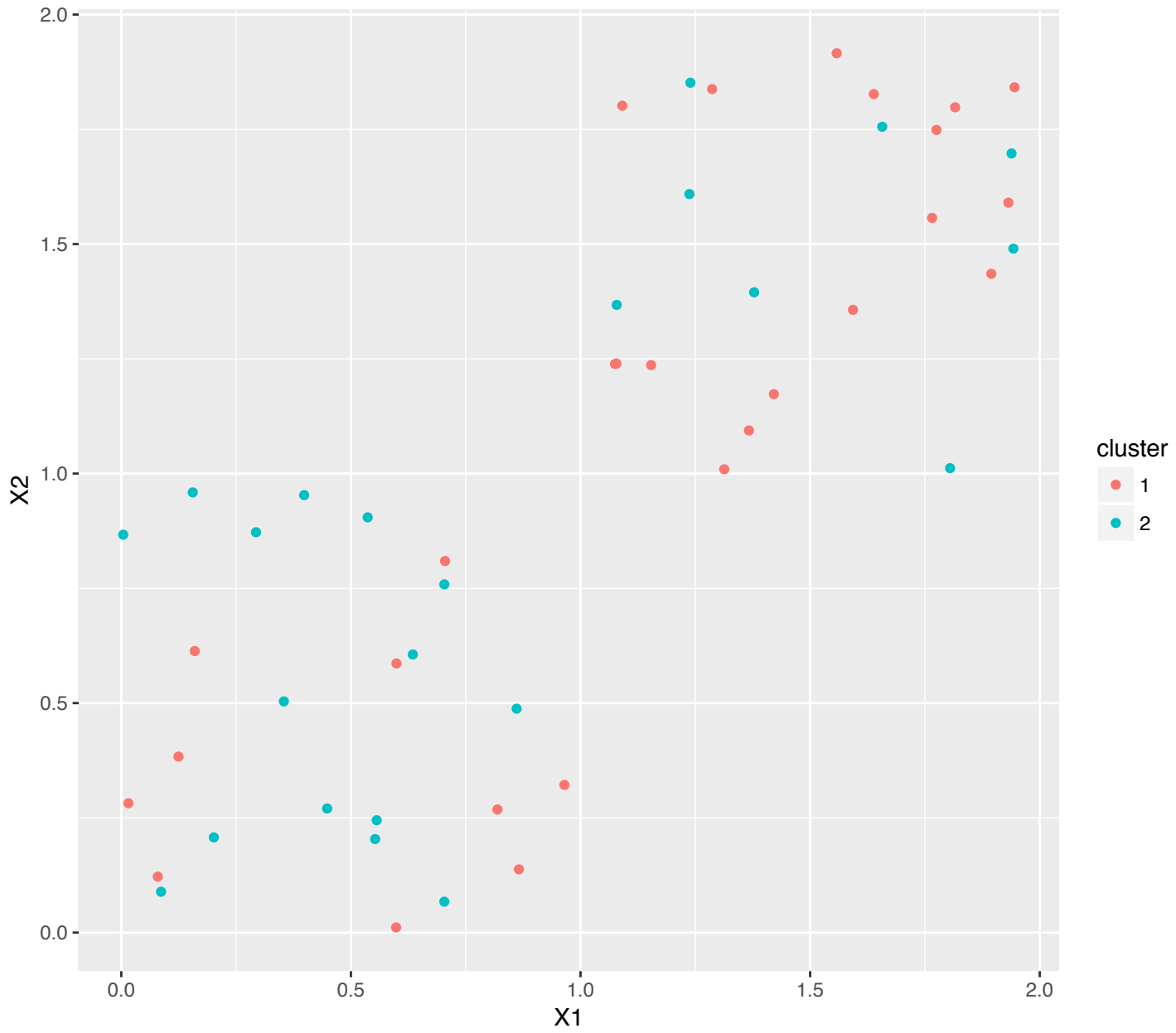
Randomly Assign 50 Points to 2 Clusters
